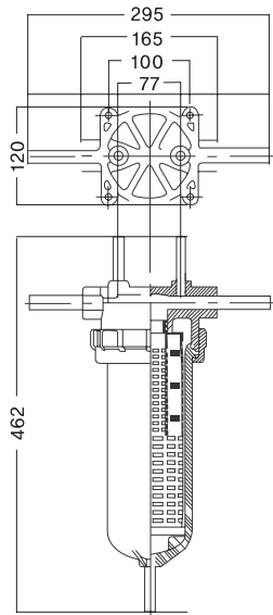
3/4 Inch NPT female connection
